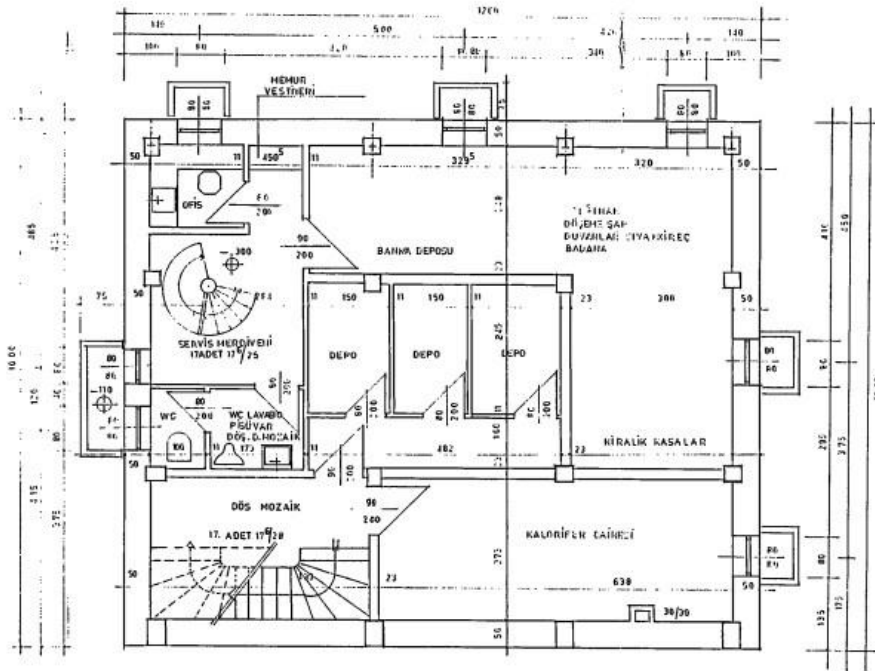
BODRUM KATI PLANI 1:50
