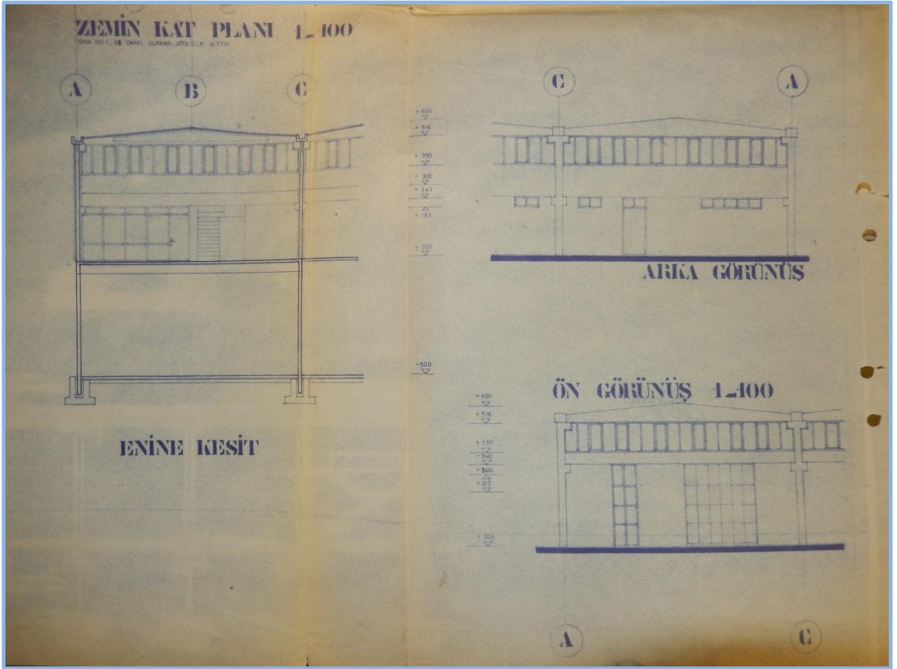
Enine Kesit
